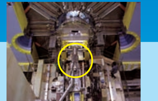
Superconducting quadrupole magnets at the interaction point: These focusing magnets compress the beams to achieve a higher rate of electron-positron collisions.
