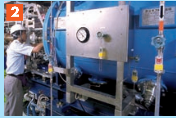
Superconducting cavity: The superconducting cavity installed in the electron ring. The cavity is made of superconducting materials, which create a high acceleration voltage. KEK's superconducting technology is among the most advanced in the world.
