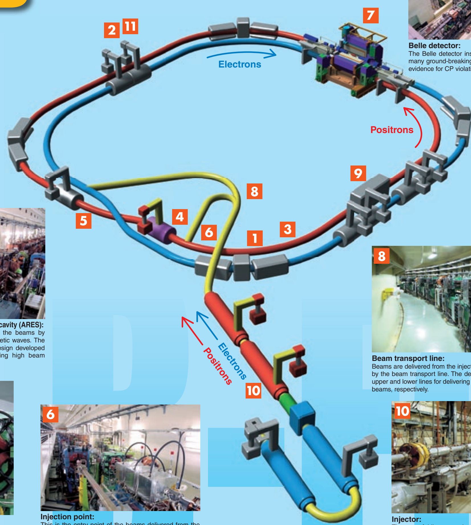
Injection point: This is the entry point of the beams delivered from the injector into the storage ring. An electromagnet installed at this point pulses the magnetic field inside at high frequency in order to efficiently feed new beams into the circulating beams in the storage ring.
