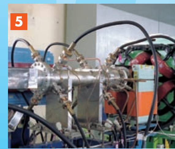
Horizontal kicker: The horizontal kicker suppresses unwanted beam oscillation in the horizontal direction while running the accelerator. The horizontal kicks are provided by radio-frequency electromagnetic waves which are transmitted via thick cables.
