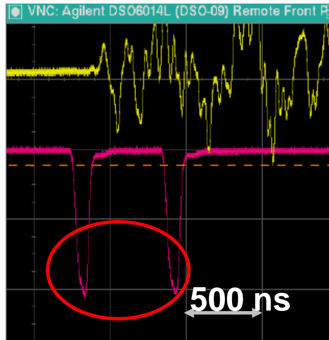
3NBT Beam Bunch Signal
