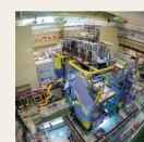
Particle and Nuclear Physics
