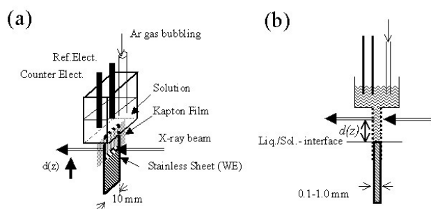
Figure 10 Schematic illustration of a newly-designed electrochemical cell conducted for in situ XAFS and XANES measurements.
