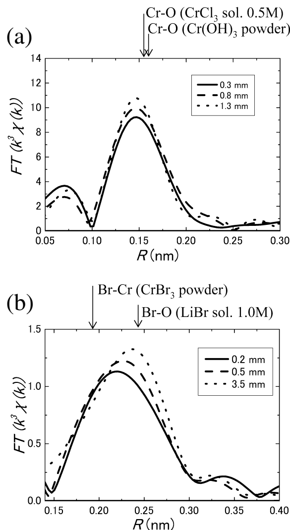
Figure 12 Fourier transforms of XAFS spectra obtained by in situ measurement at (a) Cr-K edge for d(z)=0.3, 0.8 and 1.3\text{ mm} , and (b) Br-K edge obtained by in situ measurement for d(z)=0.2, 0.5 and 3.5\text{ mm} .
