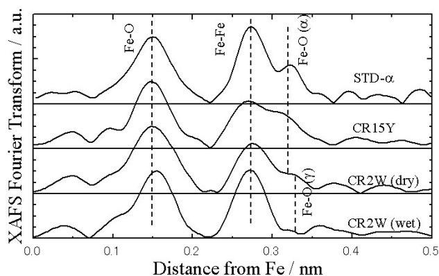
Figure 5 Radial distribution functions obtained by XAFS: (from top) crystalline \alpha -FeOOH, CR15Y, CR2W(dry), and CR2W(wet), where they are measured at Fe K-edge and symbols such as “Fe-O” show identification of peak.
