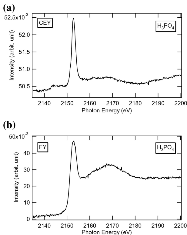
Figure 6 P K-edge XANES spectra of \text{H}_3\text{PO}_4 (a) measured with Conversion Electron Yield and (b) measured with Fluorescence Yield.
