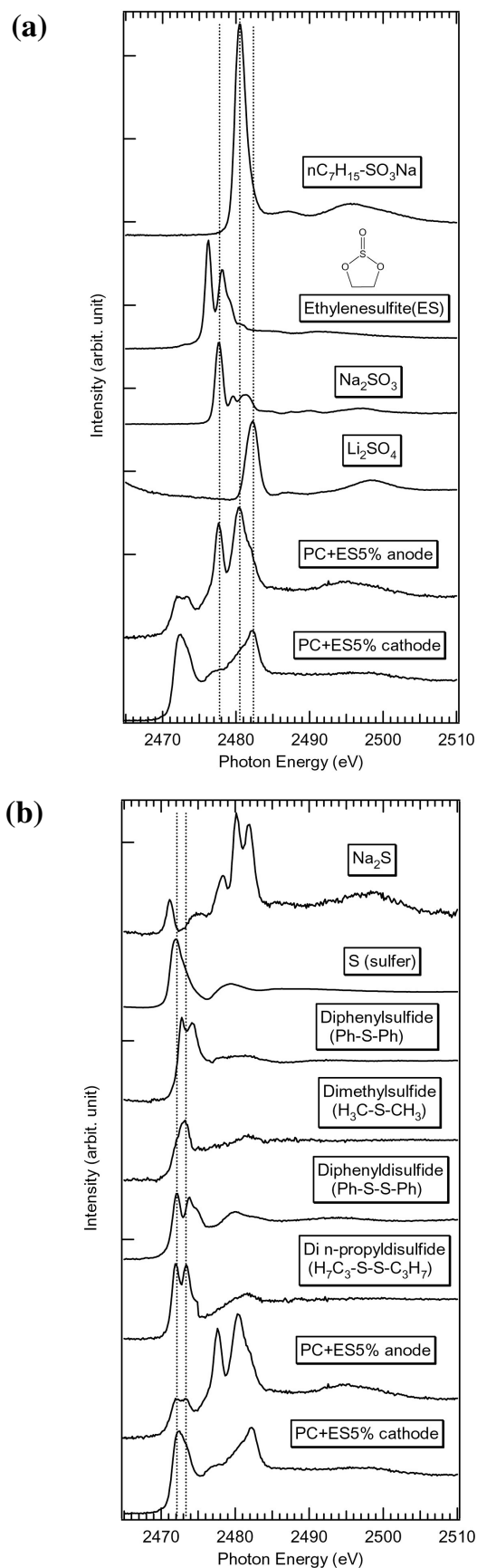
Figure 5 S K-edge XANES spectra of graphite anode and \text{LiCoO}_2 cathode compared with standard sulfur reagent. (a) \text{nC}_7\text{H}_{15}\text{-SO}_3\text{Na} , Ethylenesulfite (ES), \text{Na}_2\text{SO}_3 , \text{Li}_2\text{SO}_4 , (b) \text{Na}_2\text{S} , S (sulfur), Diphenylsulfide (Ph-S-Ph), Dimethylsulfide ( \text{H}_3\text{C-S-CH}_3 ), Diphenyldisulfide (Ph-S-S-Ph), Di n-propyldisulfide ( \text{H}_7\text{C}_3\text{-S-S-C}_3\text{H}_7 ).
