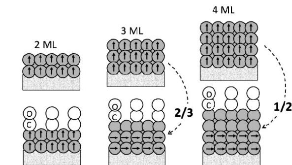
Figure 4 The schematic models of CO adsorbed Fe films. Solid arrows represent spin magnetic moment, or magnetization.
