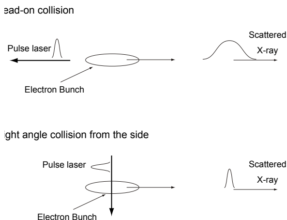
Figure 1 Schematic figures of laser inverse Compton scattering by a head-on collision and collision from the right angle from the side.
