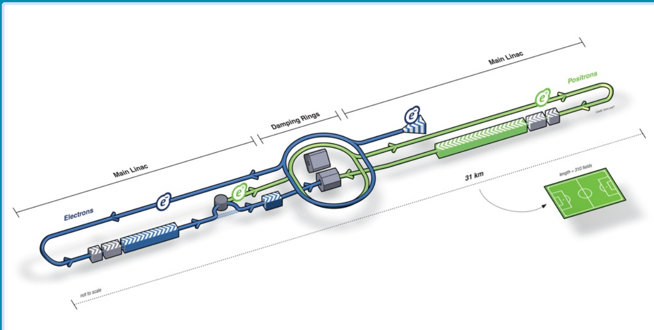
ILC : Facing each other, two linear accelerators - one for electrons and other for positron - will stretch total of approximately 31 km. Like any complex machine, ILC is made up of several systems - each one an essential component for launching particles at close to the speed of light. (Graphic courtesy of ILC / form one visual communication)
