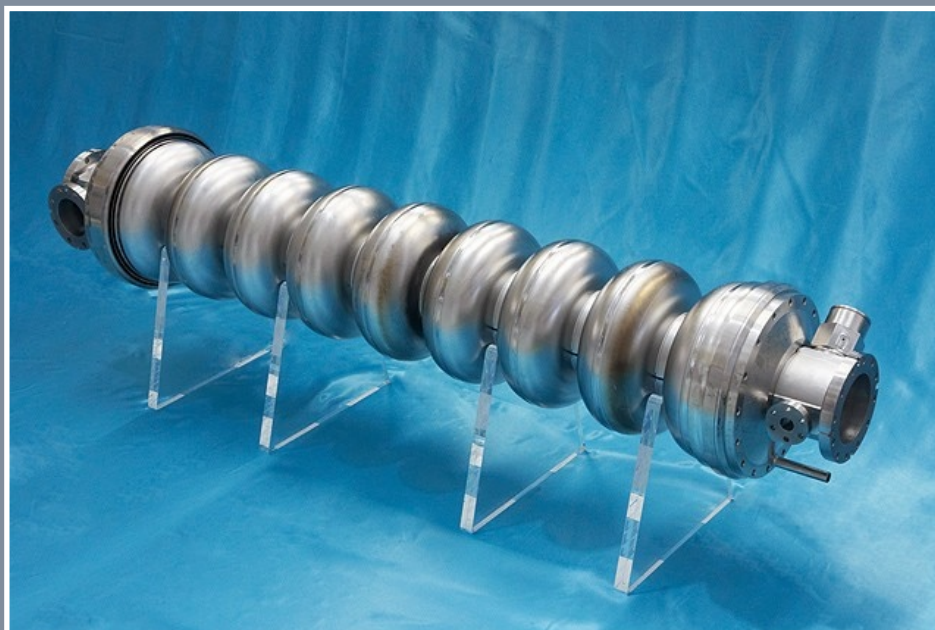
The one meter-long superconducting accelerating cavities are made from nine cells, polished to provide micro-level surface smoothness, and free of impurities. A series of detailed chemical treatments and processes make the cavity literally sparkle. (Photo by Nobu Toge)
